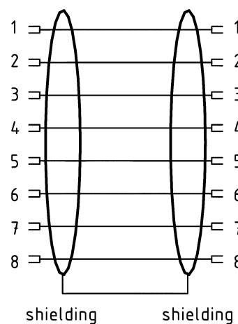
schematic diagram
