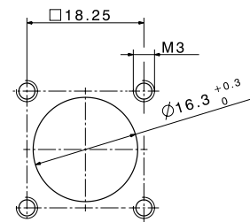
hole pattern
